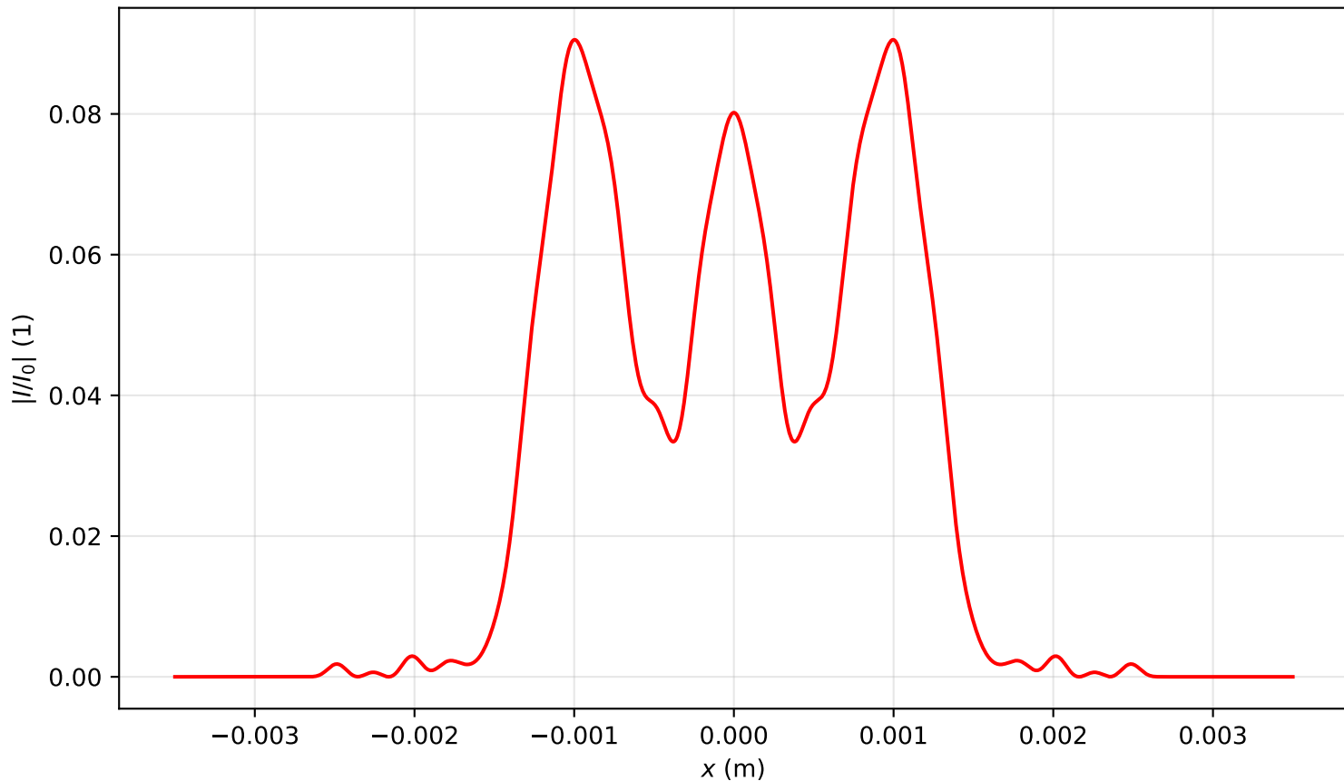
Intensity profile I(x, y = 0, z = 2.627)/I_0 , P_{in}=6.5P_{cr} , artificial time
